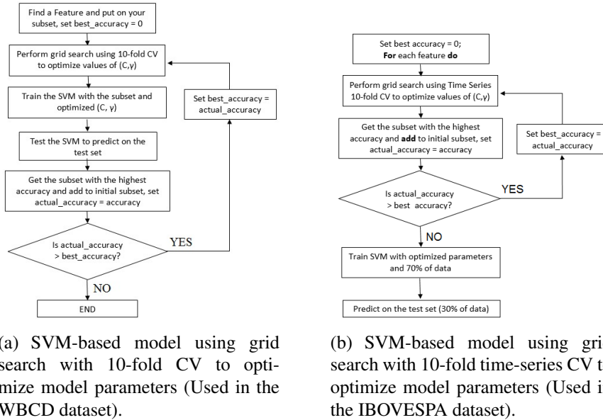
Figure 5. Processes used to evaluate the datasets.
