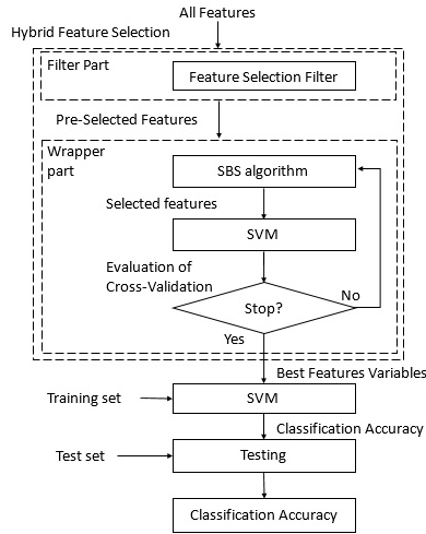
Figure 3. A Hybrid feature selection method, adapted from [Lee 2009].
