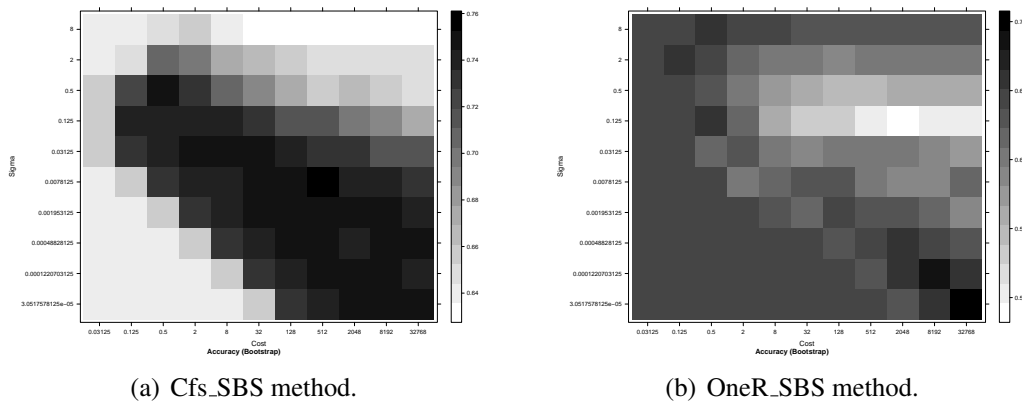
Figure 6. Values of Grid-Search optimization for RBF kernel ( C, \gamma ) and IBOVESPA dataset.
