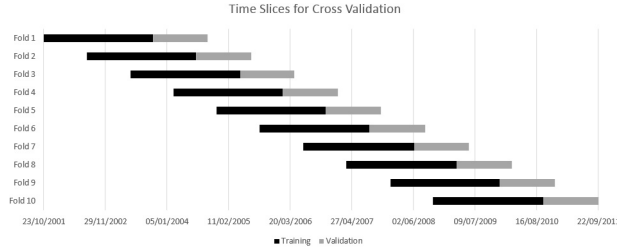
Figure 4. 70% of IBOVESPA dataset sliced at 10-fold for cross-validation.
