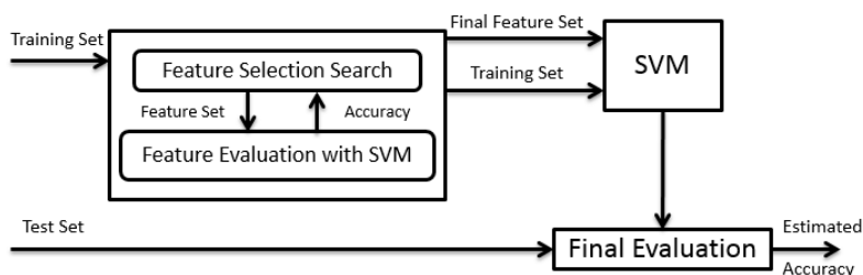
Figure 1. Wrapper model, adapted from [Kohavi and John 1997].
